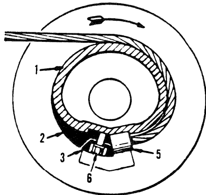
OVERWINDING
