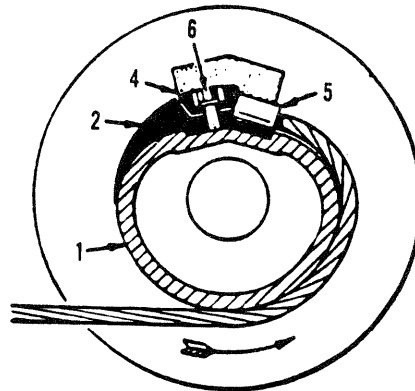
UNDERWINDING
