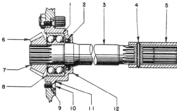
STANDARD SPEED WINCH 46.1:1 GEAR RATIO
