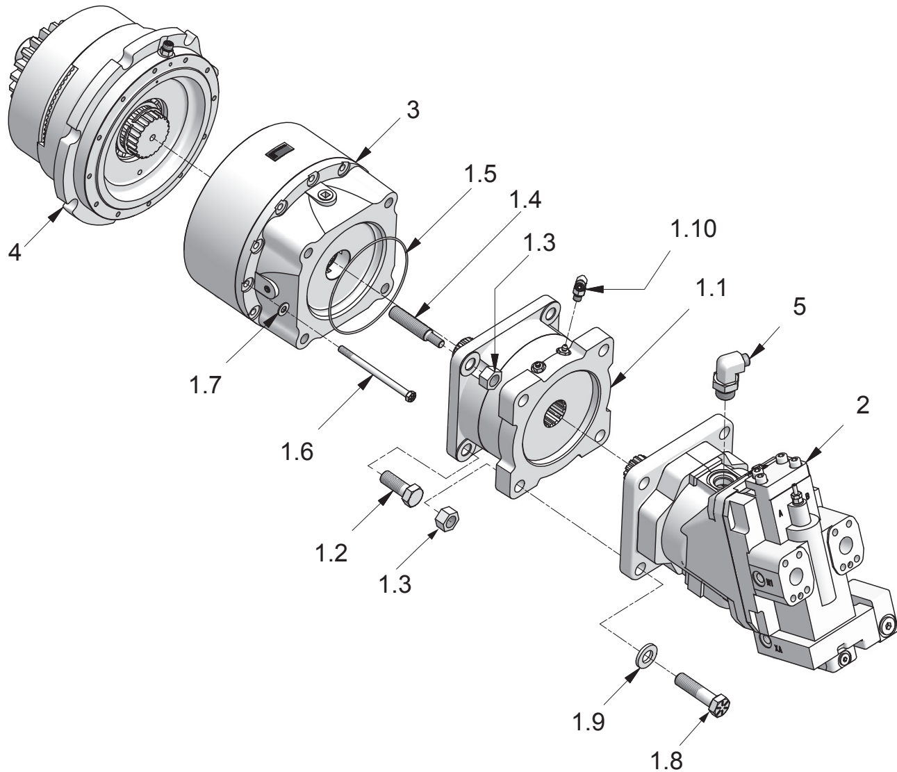
Motor Shaft Assy Case Quadtrac (H6HH6BN**R39)
