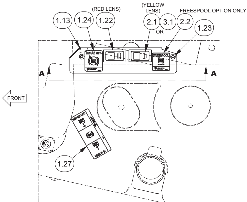
CONTROLS INSTALLATION TOP VIEW (FREESPOOL OPTION SHOWN)
