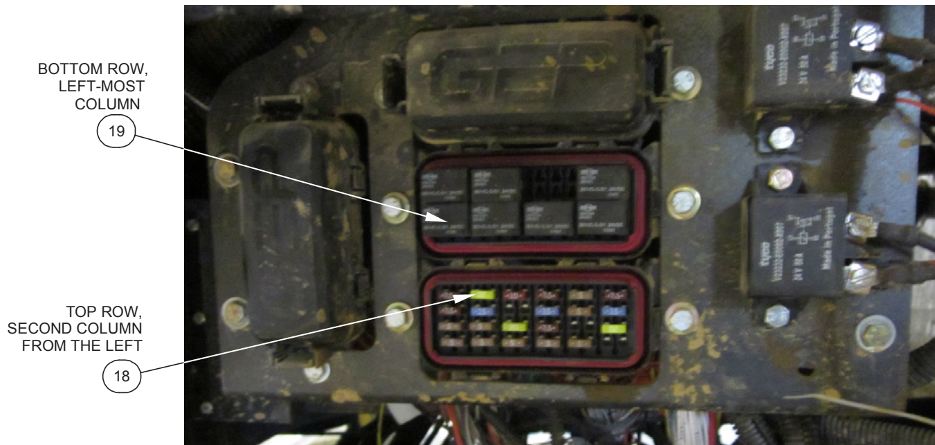
ELECTRICAL PANEL LEFT SIDE ACCESS PANEL
