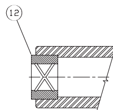
CURRENT DESIGN
