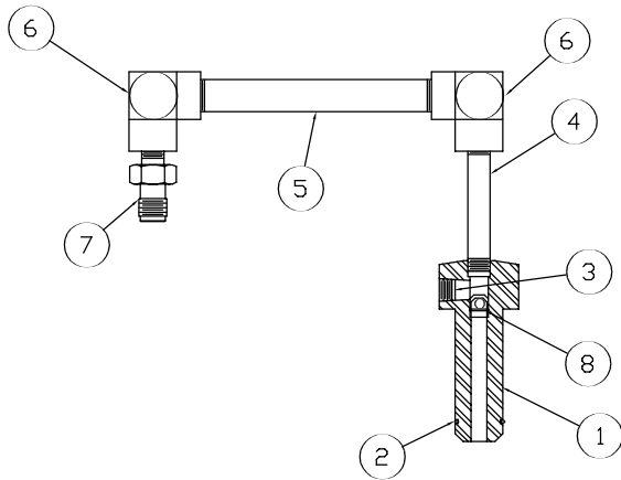
81823 4-Shaft, Brake Side (Older Units - Prior to Dec 1995)
