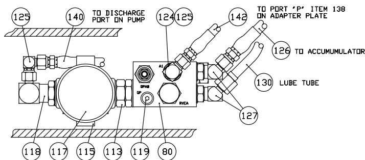
DETAIL G
