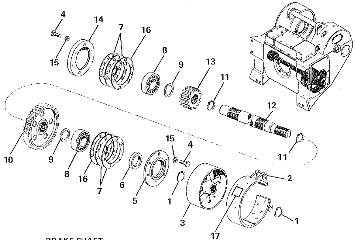
BRAKE SHAFT
