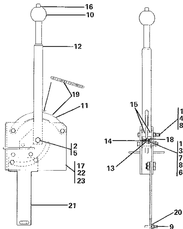
BRAKE STAND — NO. 49434
