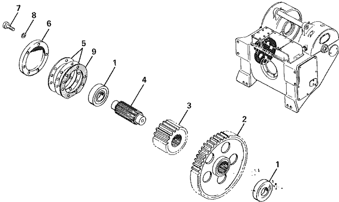
IDLER SHAFT (NO FREE SPOOL)
